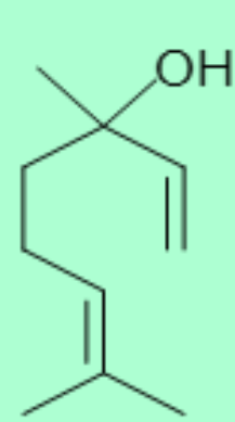
Linalool
