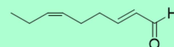
(E,Z)-2,6-Nonadienal
