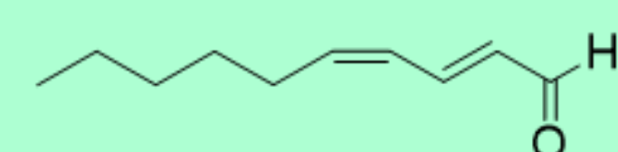
(E,Z)-2,4-Decadienal
