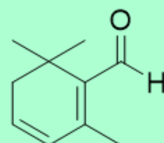
Safranal
