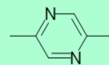
2,5-Dimethylpyrazine
