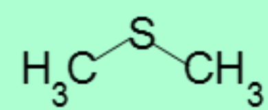
Dimethylsulfide
