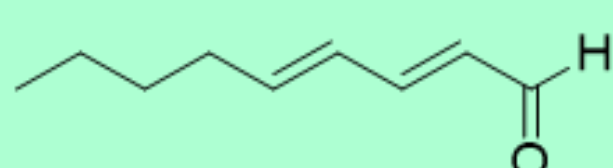
(E,E)-2,4-Nonadienal
